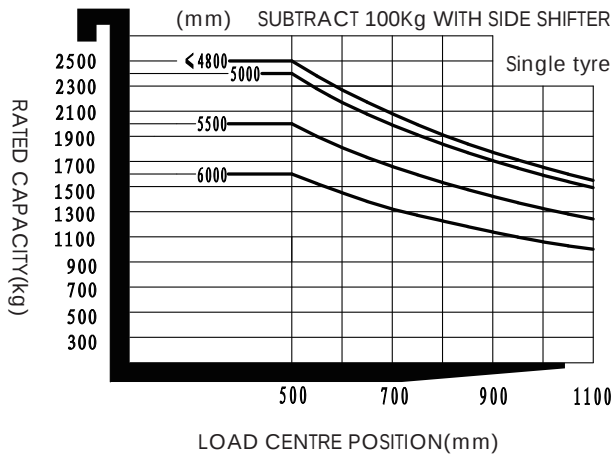
RATED CAPACITIES AND LOAD CENTERS GRAPH
